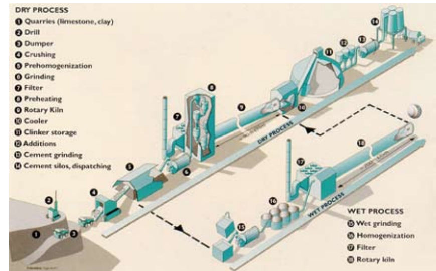
Figure 3.a Portland cement dry and wet manufacturing processes [41]
