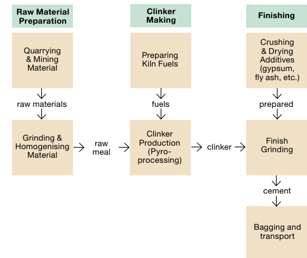
Figure 3.a Portland cement dry and wet manufacturing processes [41]
