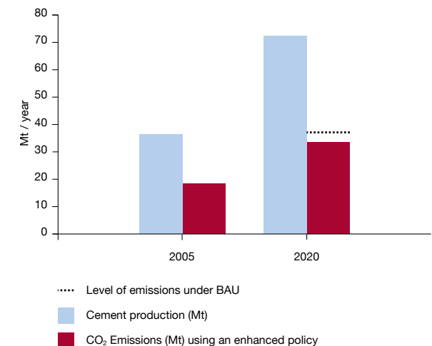
Figure 4.a Production and emission scenario for Brazil
